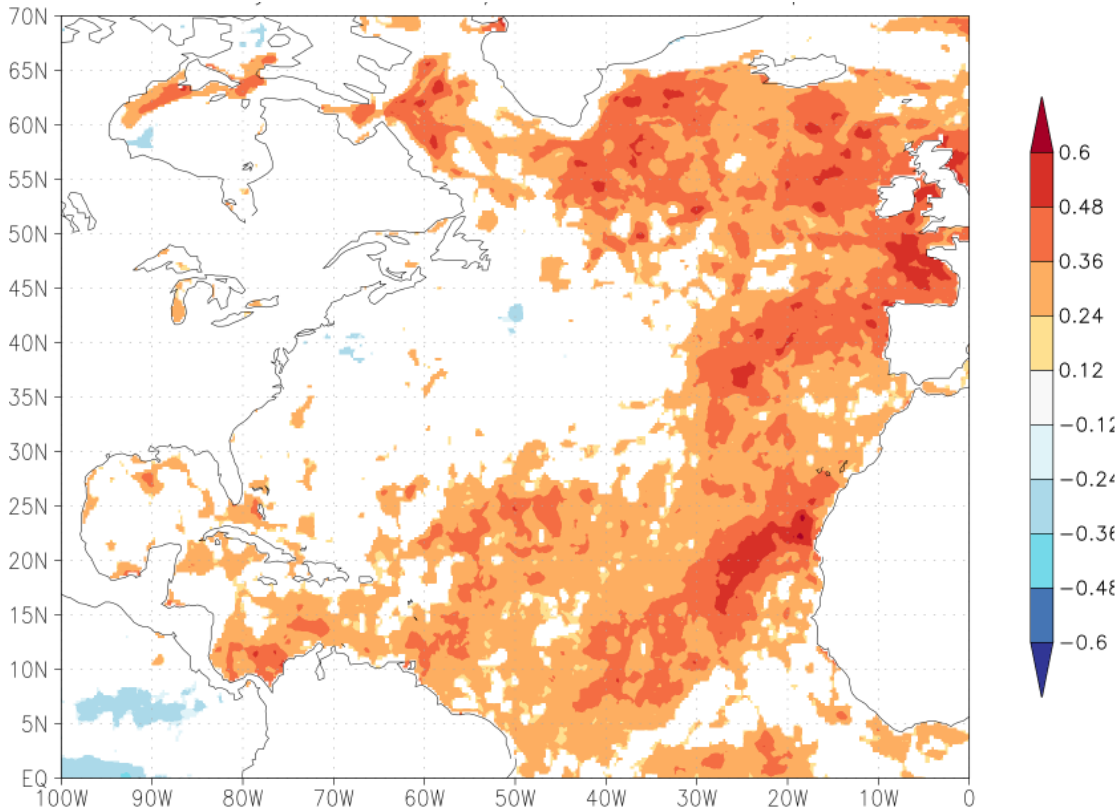
Figure 24: Rank correlation between May North Atlantic SST anomalies and seasonal Atlantic ACE from 1982-2019.
