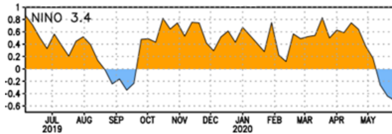
Figure 13: Nino 3.4 SST anomalies from June 2019 through May 2020. Figure courtesy of Climate Prediction Center.
