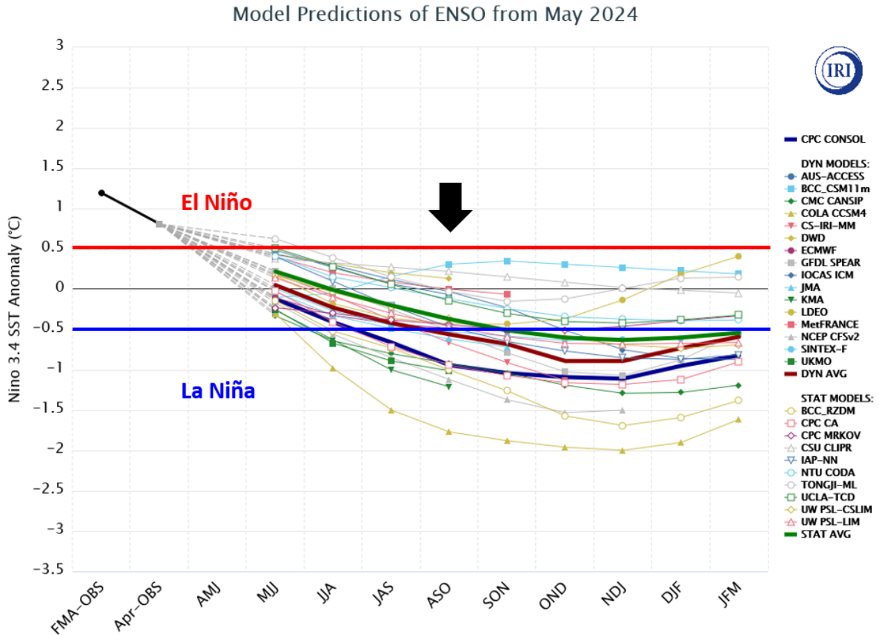
Figure 24: ENSO forecasts from various statistical and dynamical models for Nino 3.4 SST anomalies based on late April to early May initial conditions. All models call for either ENSO neutral or La Niña conditions for August–October. The black arrow delineates the peak of the Atlantic hurricane season (August–October). Figure courtesy of the International Research Institute (IRI).
