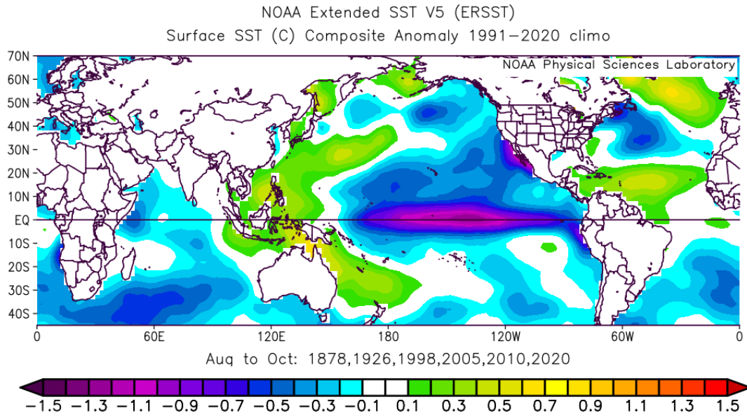
Figure 11: Average August–October SST anomalies in our six analog years.
