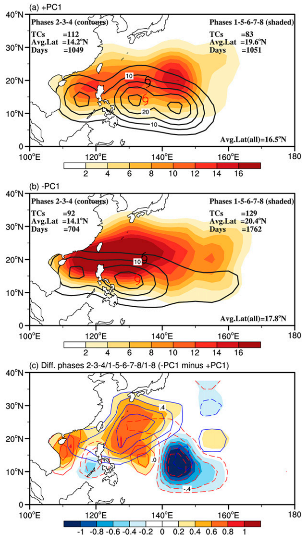
FIG. 6. Spatial distribution of TC genesis frequency for phases 2–4 (contours) and phases 1 and 5–8 (shaded) for years with (a) PC1 greater than 0 and (b) PC1 less than 0. The corresponding TC genesis frequency, the average TC genesis latitude, and the frequency of occurrence for phases 2–4 (phases 1 and 5–8) are shown in the top left (top right). The bottom-right value is the average latitude for all eight phases. (c) Difference of TC genesis distribution for BSISO phases 2–4 (red contours), phases 1 and 5–8 (blue contours), and all eight BSISO phases (shaded) between strong negative PC1 and positive PC1 years.
